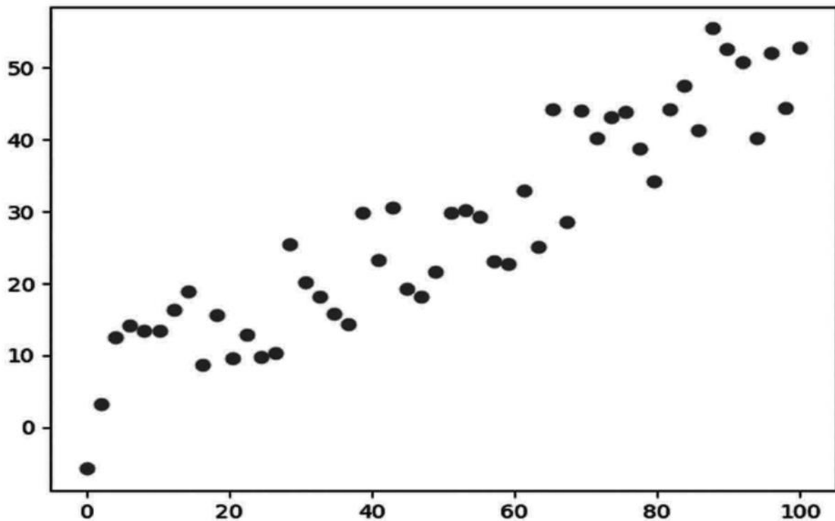
Fig. 9.1 Program Output
